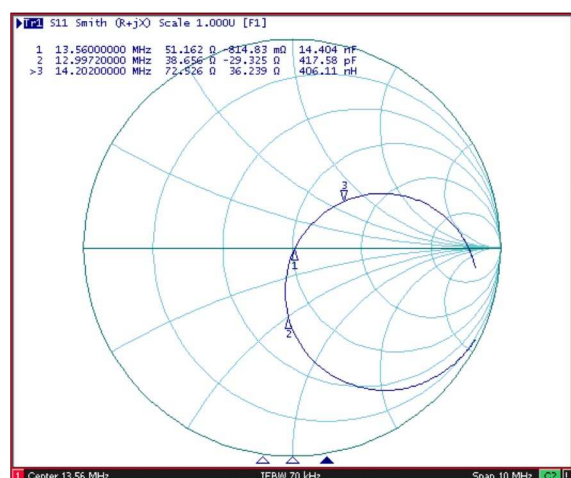
Figure 13. Lower Q Antenna Measurement Plots with Calculated Values ( Q \approx 10 )
