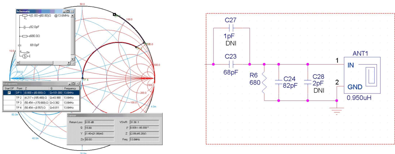
Figure 9. Smith Chart Simulation ( R_{PAR} = 680 \Omega )
