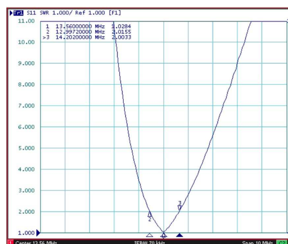
Figure 13. Lower Q Antenna Measurement Plots with Calculated Values ( Q \approx 10 )
