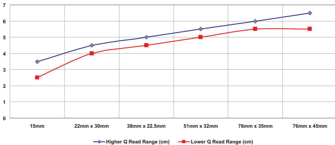
Figure 16. ISO14443B Transponder Read Ranges with TRF7960TB
