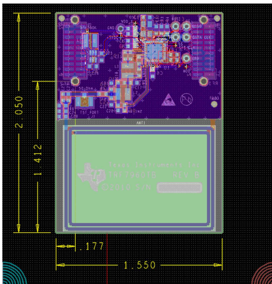
Figure 7. Mechanical/Physical Information
