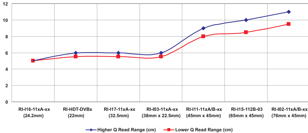
Figure 14. ISO15693 Transponder Read Ranges with TRF7960TB
