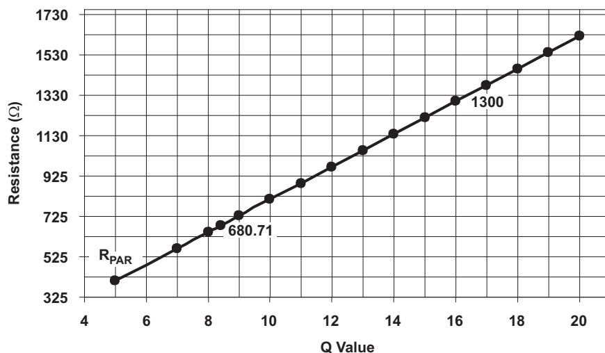
Figure 10. Theoretical Parallel Resistor Value for Desired Q
