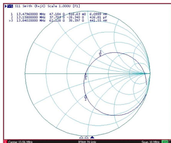
Figure 12. Higher Q Antenna Measurement Plots with Calculated Values ( Q \approx 20 )
