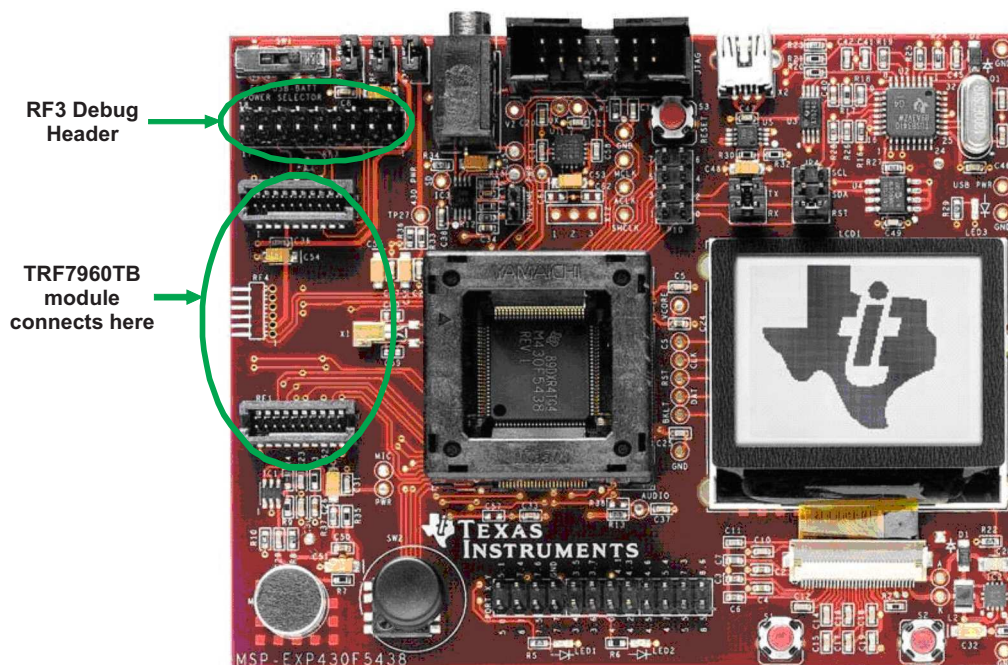
Figure 3. MSP-EXP430F5438 Development Board
