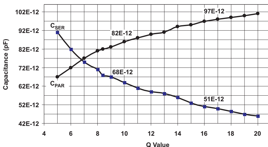
Figure 11. Theoretical Capacitance Values for Resonance at Desired Q
