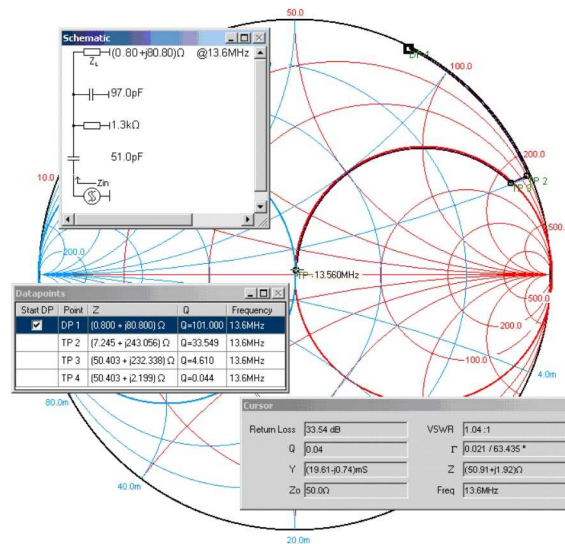
Figure 8. Smith Chart Simulation ( R_{PAR} = 1.3 k \Omega )
