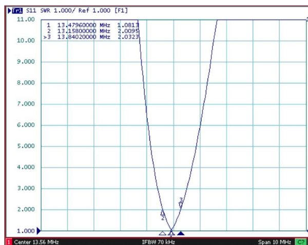
Figure 12. Higher Q Antenna Measurement Plots with Calculated Values ( Q \approx 20 )
