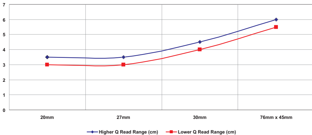
Figure 15. ISO14443A Transponder Read Ranges with TRF7960TB
