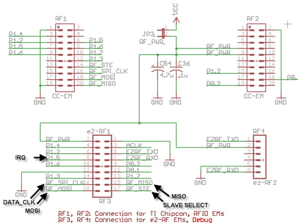
Figure 4. Debug Header (RF3) Logic Analyzer Connections for Monitoring SPI Communications Between MSP430F5438A and TRF796x on TRF7960TB Module
