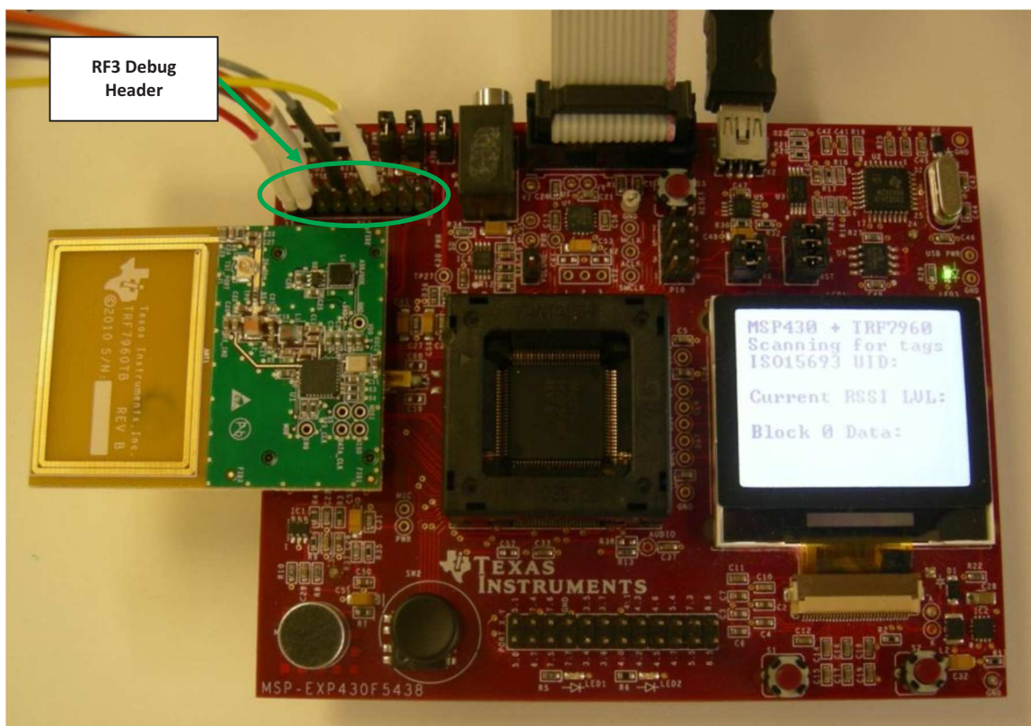
Figure 5. Firmware Development\Debug Setup for MSP-EXP430F5438 Experimenters Board
