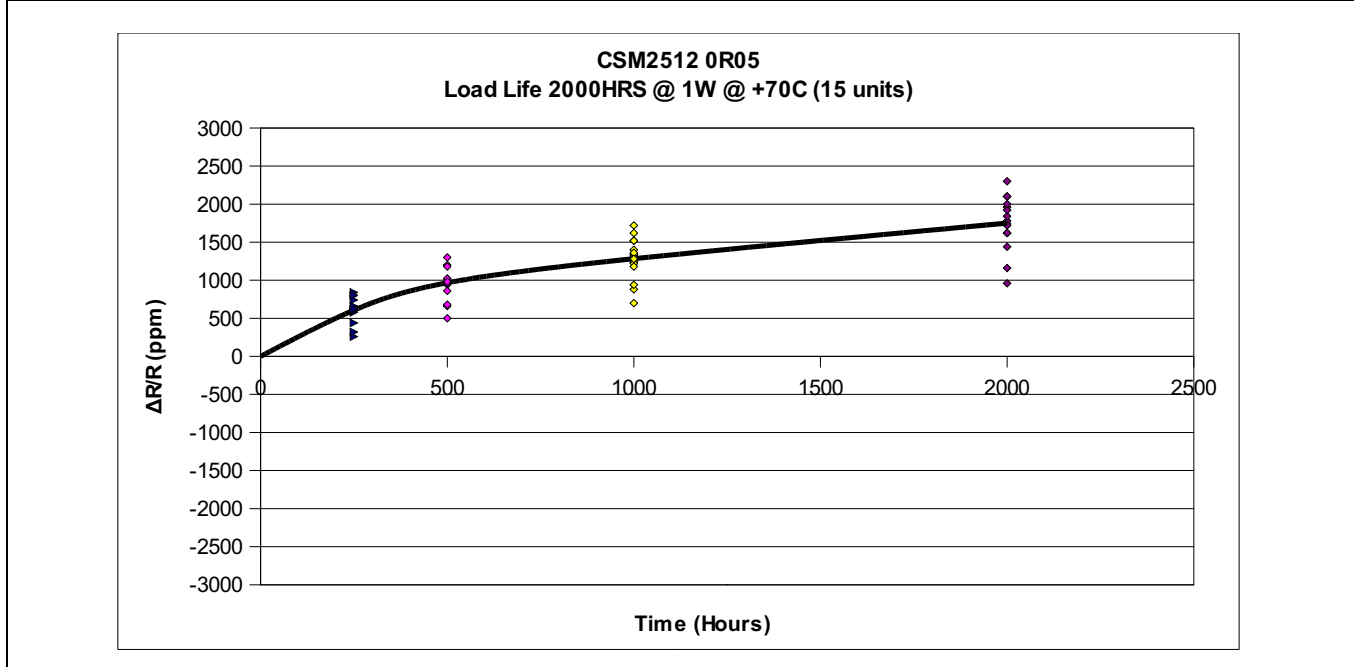
FIGURE 3 - LOAD LIFE RESULTS OF CSM2512
