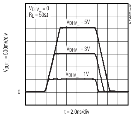
DRIVER LARGE-SIGNAL RESPONSE
