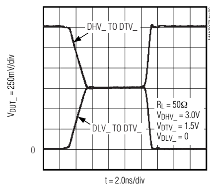
DRIVE TO TERM TRANSITION
