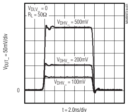
DRIVER SMALL-SIGNAL RESPONSE
