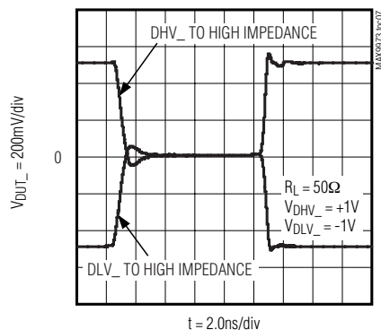
DRIVE TO HIGH IMPEDANCE TRANSITION
