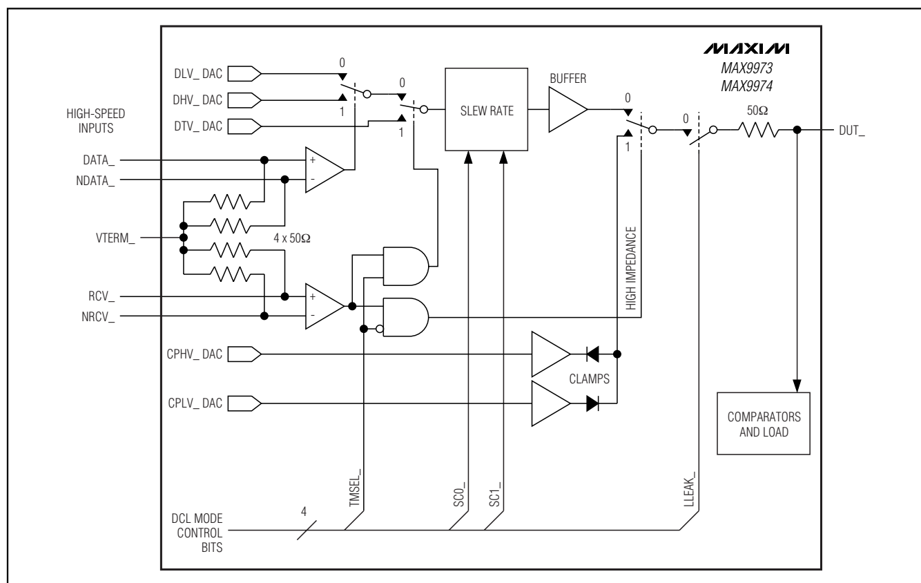
Figure 2. Simplified Driver Channel
