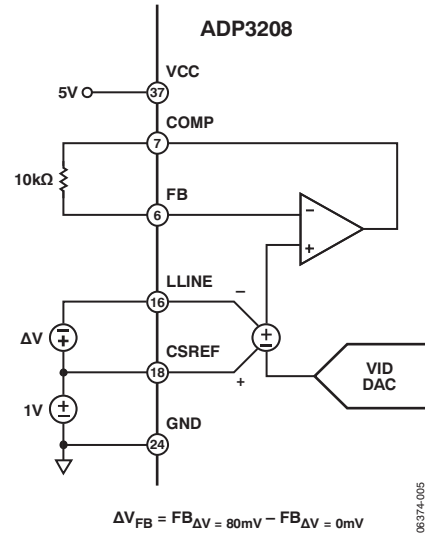
Figure 6. Positioning Accuracy
