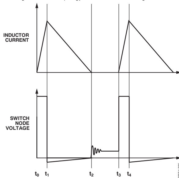
Figure 34. Inductor Current and Switch Node in DCM
