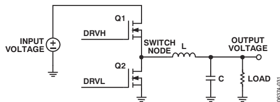
Figure 30. Buck Topology
