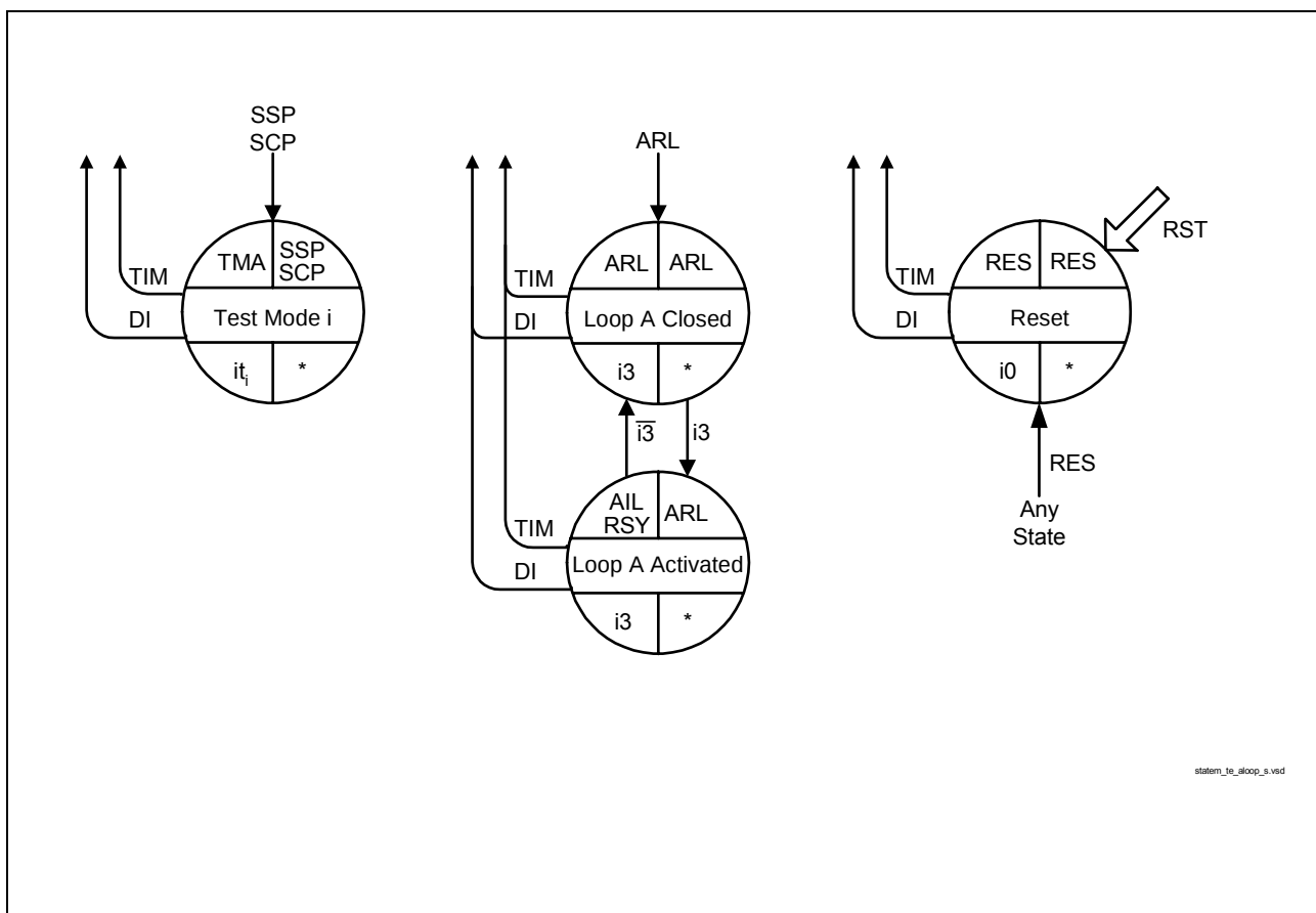
Figure 40 State Transition Diagram of Unconditional Transitions (TE, LT-T)
