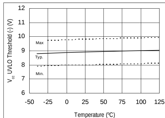
Figure 17. V cc Undervoltage Threshold (-) vs. Temperature
