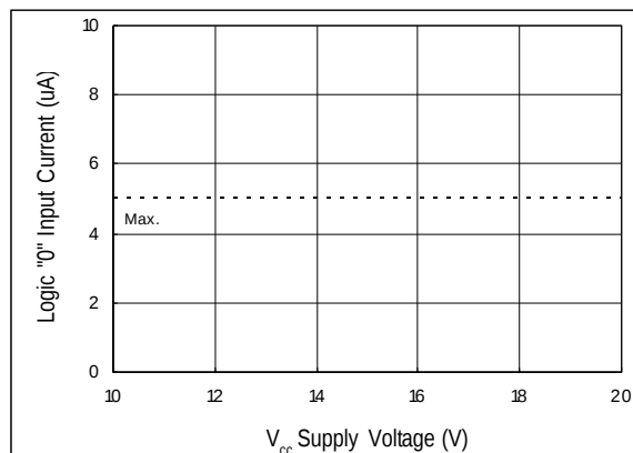
Figure 15B. Logic "0" Input Current vs. Supply Voltage
