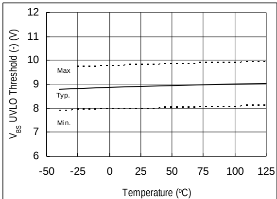
Figure 19. V BS Undervoltage Threshold (-) vs. Temperature
