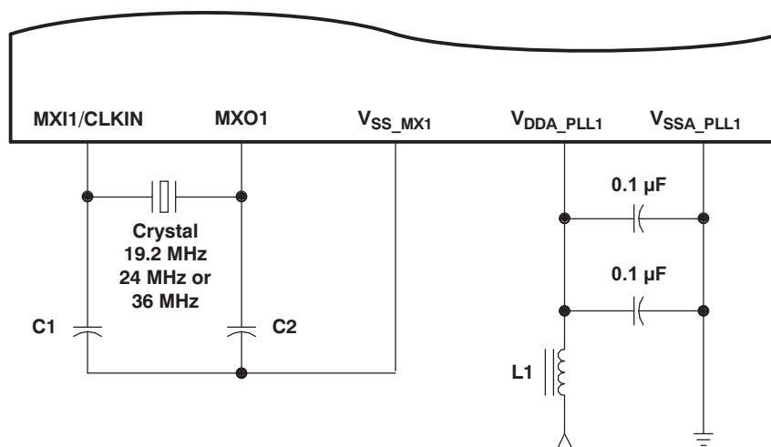
Figure 6-5. MXI1 Oscillator
