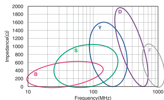
MMZ1005 Type
