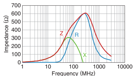
MMZ1608Y102B
