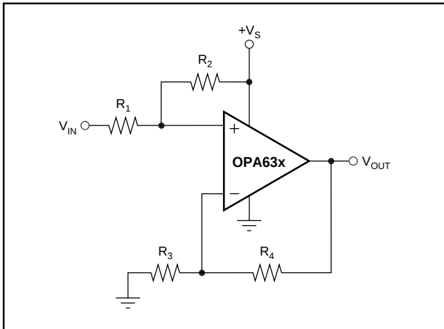
FIGURE 3. DC Level-Shifting Circuit.
