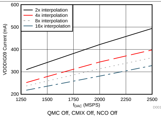
Figure 39. VDDD/G09 Current vs f_{\text{DAC}} Over Interpolation
