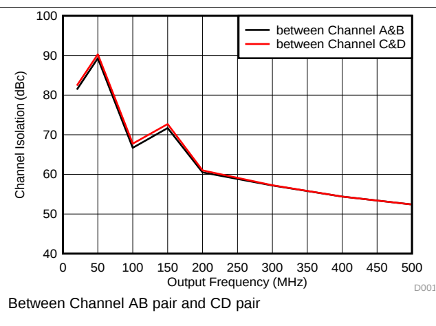
Figure 30. Channel Isolation
