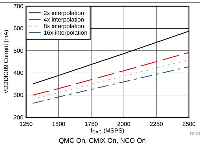
Figure 41. VDDD/G09 Current vs f_{\text{DAC}} Over Interpolation
