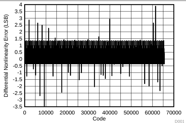
Figure 2. Differential Nonlinearity
