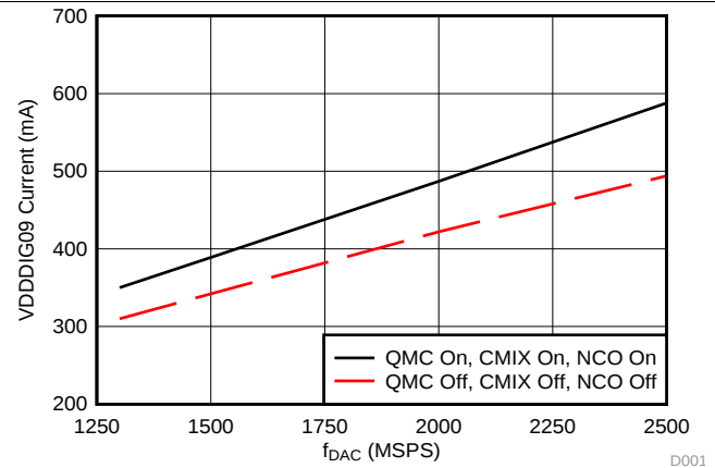
Figure 38. VDDD/G09 Current vs f_{\text{DAC}} Over Digital Processing Functions
