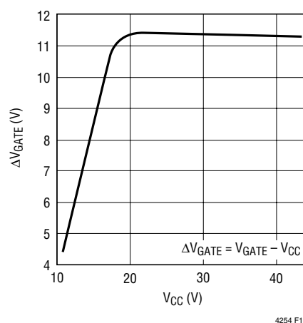
Figure 13. \Delta V_{GATE} vs V_{CC}
