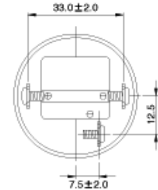
Bottom View 2
