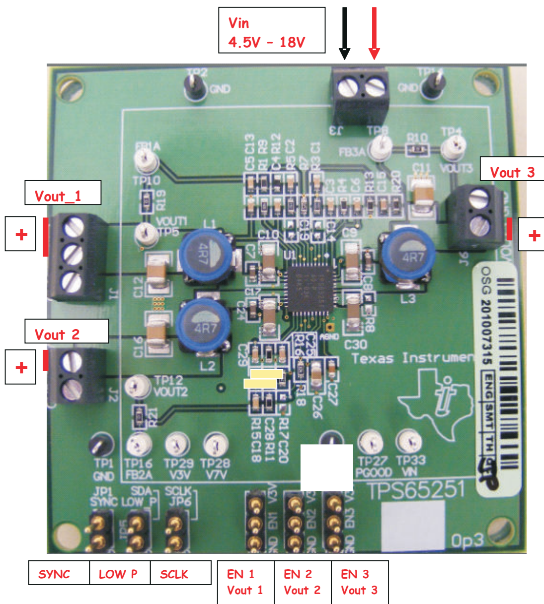
Figure 5-1. Headers Description and Jumper Placement
