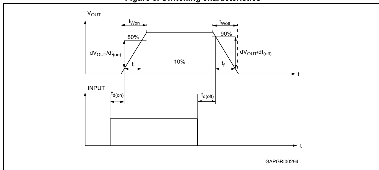
Figure 5. Switching characteristics
