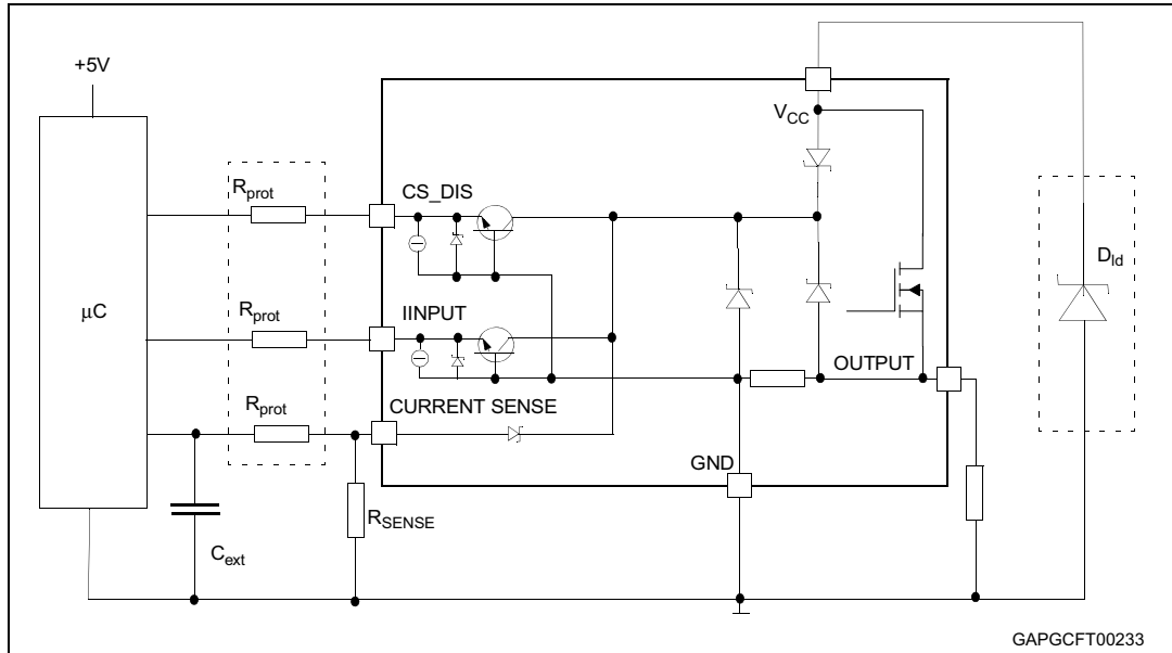
Figure 22. Application schematic
