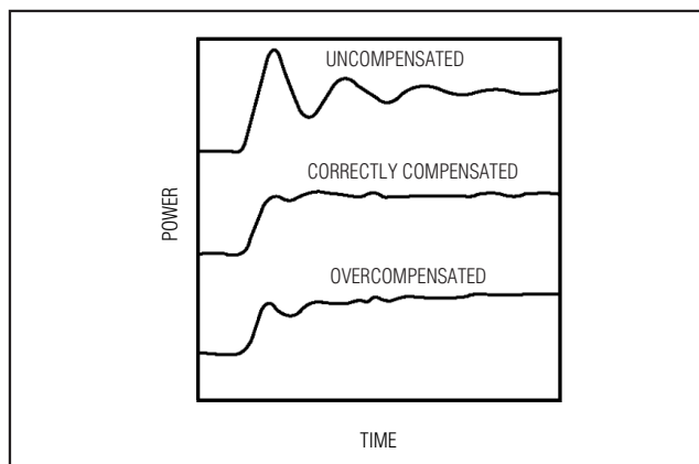
Figure 7. Laser Compensation
