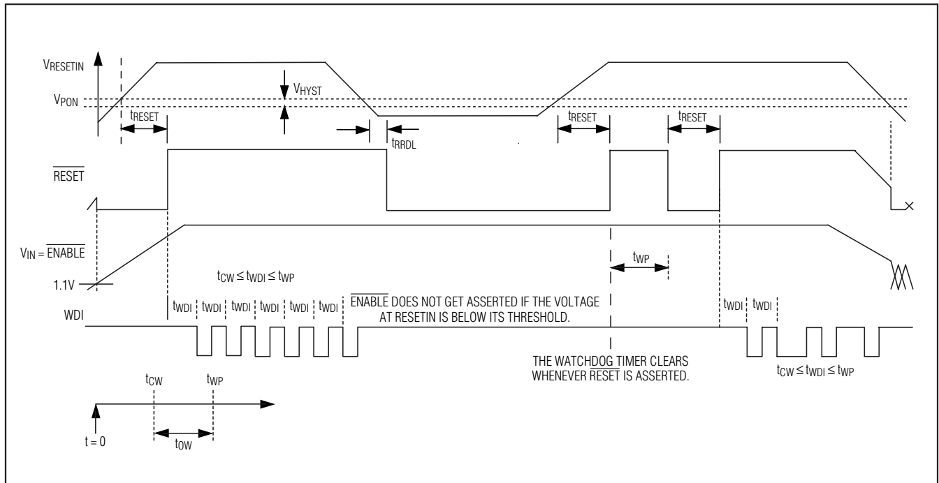
Figure 4. \overline{RESETIN} , \overline{RESET} , V_{IN} , \overline{ENABLE} , and WDI Voltage Monitoring
