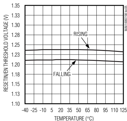
RESET/EN THRESHOLD VOLTAGE vs. TEMPERATURE
