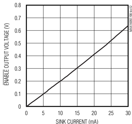
ENABLE OUTPUT VOLTAGE vs. SINK CURRENT
