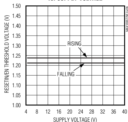
RESET/EN THRESHOLD VOLTAGE vs. SUPPLY VOLTAGE
