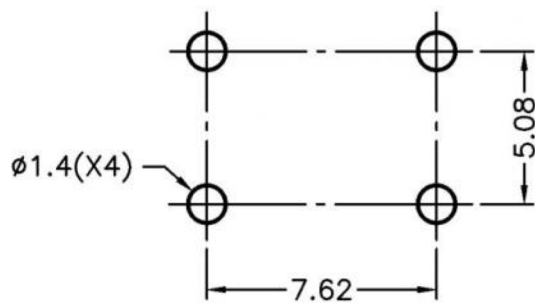
MOUNTING HOLES
