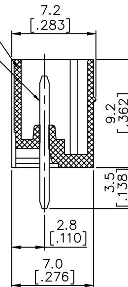
SECTION P-P
