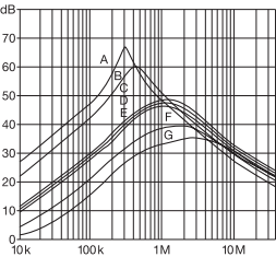
EV/EH 20 types
