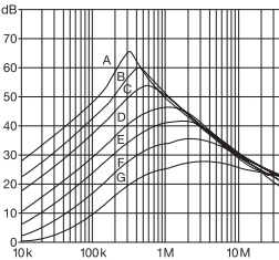
EV/EH 24 types
