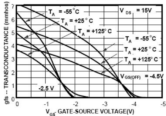
Transconductance Characteristics
