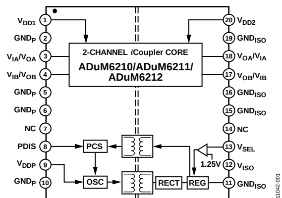
Figure 1. ADuM6210/ADuM6211/ADuM6212
