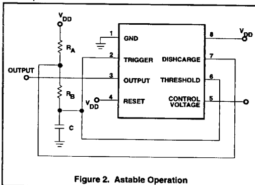
Figure 2. Astable Operation
