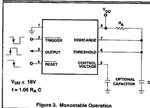
Figure 3. Monostable Operation
