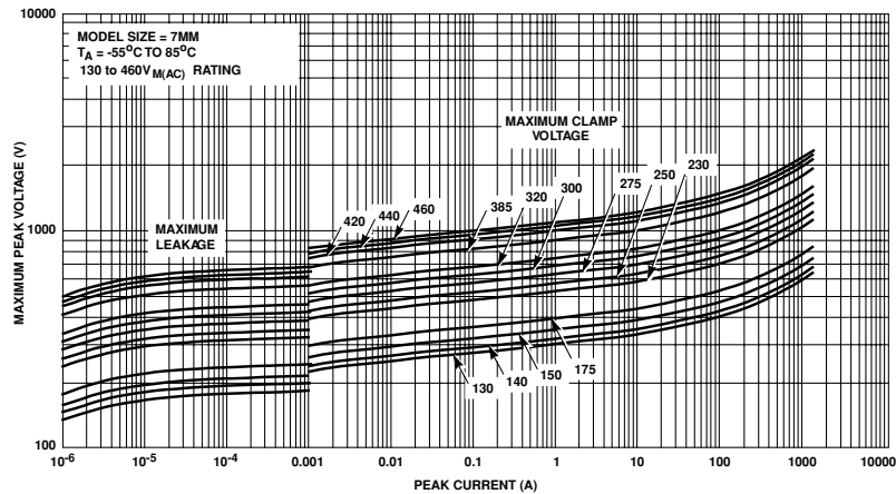
V7E130(P)-V7E460(P)
