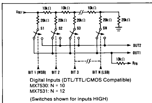
Figure 1. MX7530/MX7531 Functional Diagram
