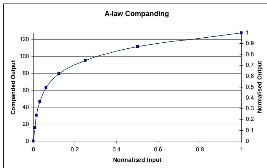
Figure 42 A-Law Companding
