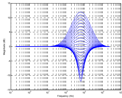
Figure 62 EQ Band 3 – Peak Filter Centre Frequencies, EQ3F Figure 63 EQ Band 3 – Peak Filter Gains for Lowest Cut-off Frequency, EQ3BW=0
