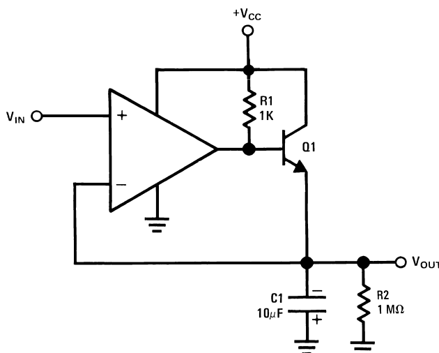
Figure 19. Positive Peak Detector
