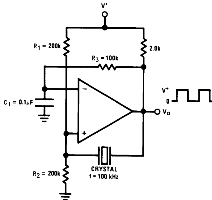
Figure 17. Crystal controlled Oscillator
