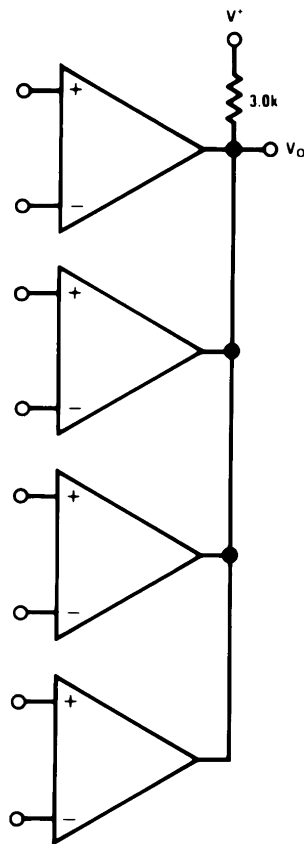
Figure 25. ORing the Outputs
