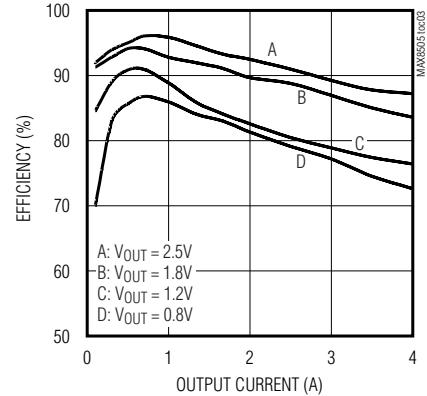
EFFICIENCY vs. OUTPUT CURRENT ( V_{IN} = V_{CC} = 3.3V , f_{SW} = 1MHz )
