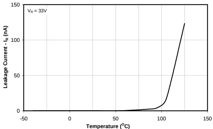
Typical Leakage Current vs Temperature
