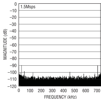
748kHz Sine Wave 4096 Point FFT Plot
