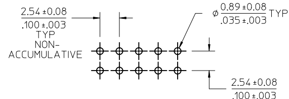
RECOMMENDED P.C. BOARD HOLE LAYOUT SCALE 4:1
