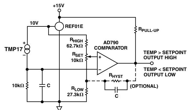
Figure 12. Variable Temperature Thermostat
