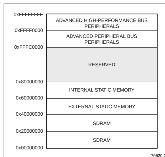
Figure 6. Memory Remap '01'
