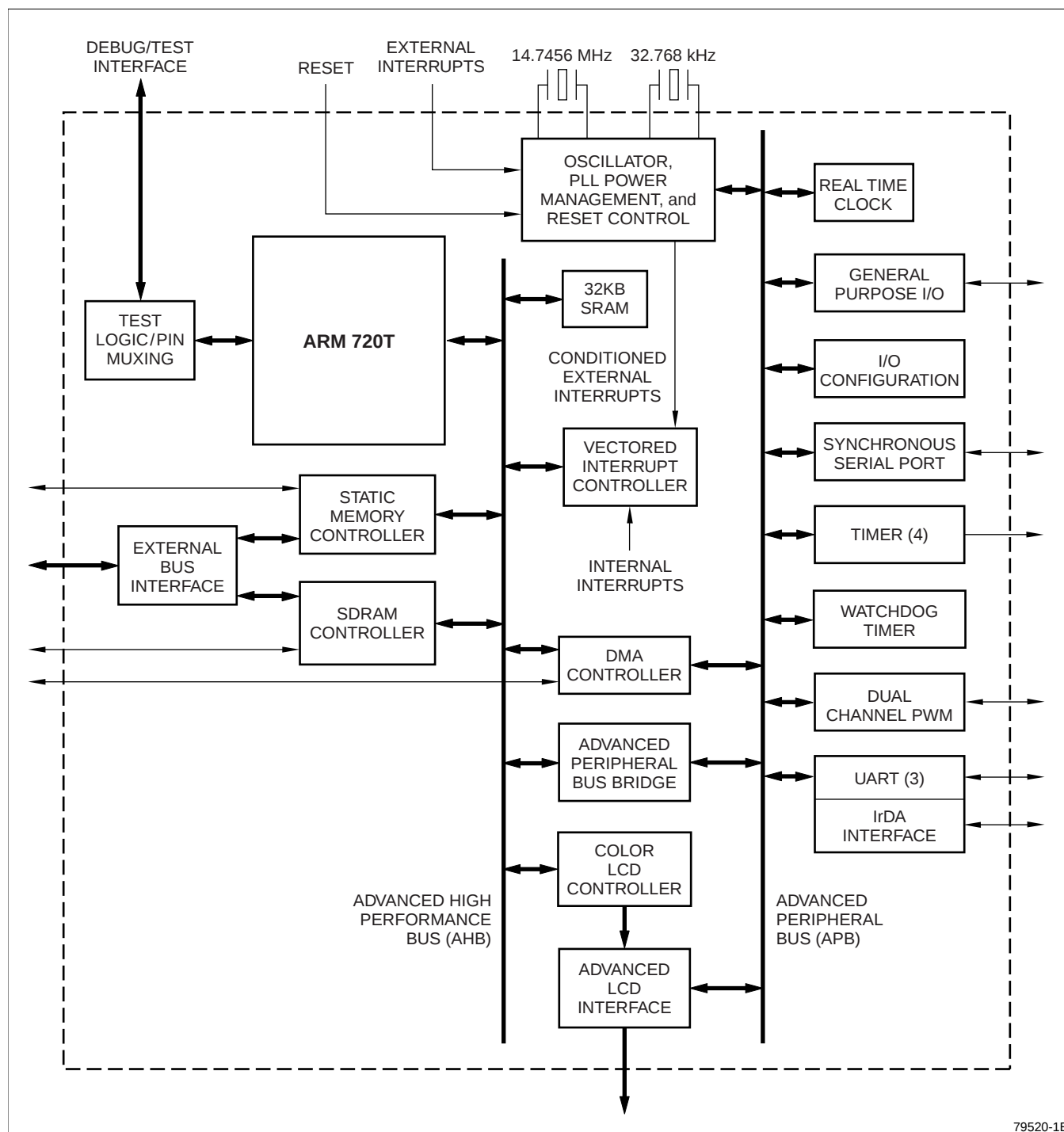
Figure 1. LH79520 block diagram
