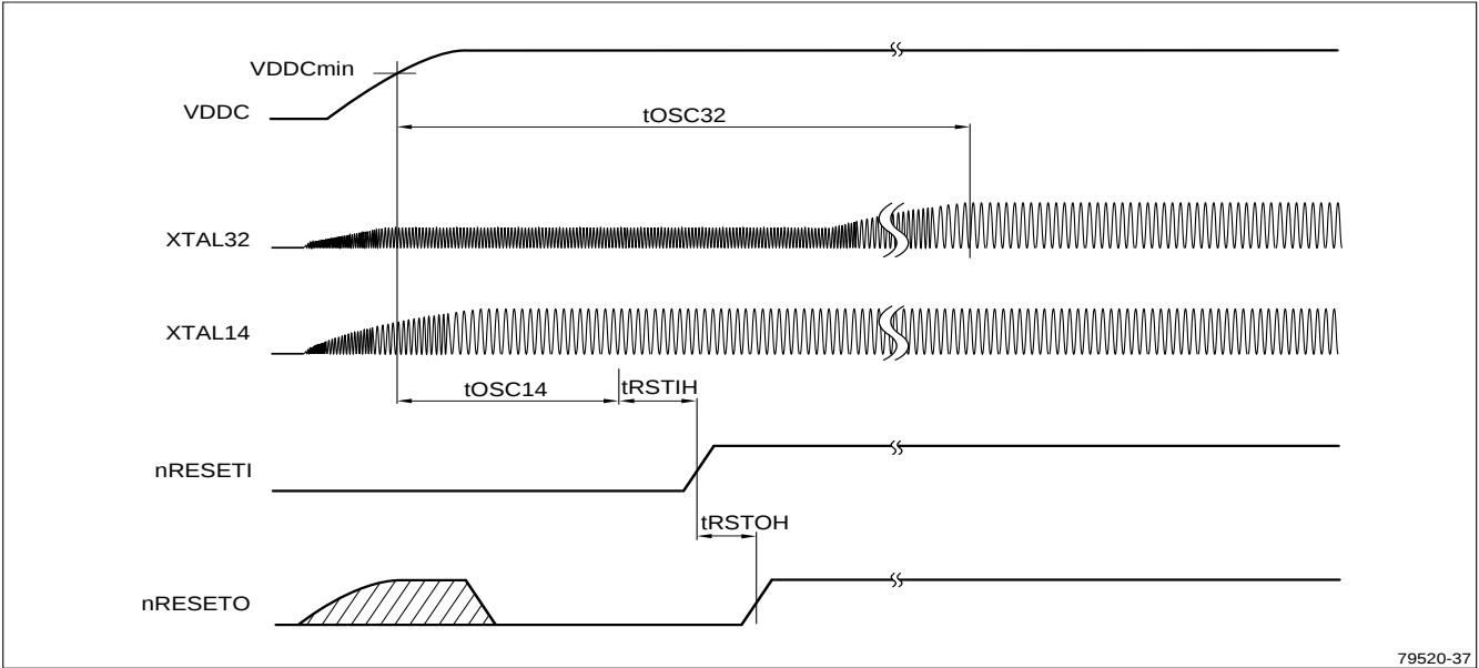
Figure 29. PLL Start-up
