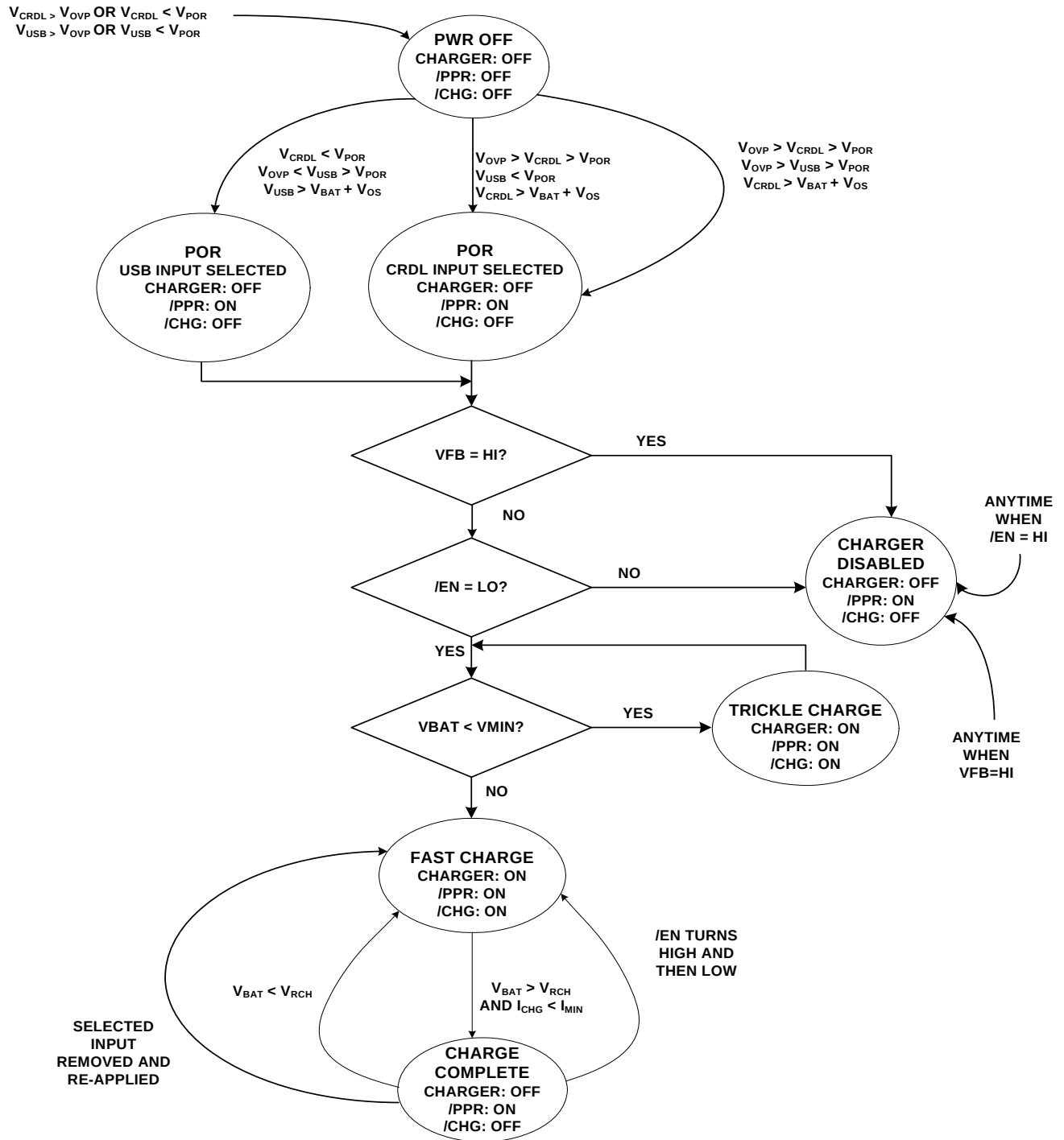
FIGURE 12. STATE DIAGRAM
