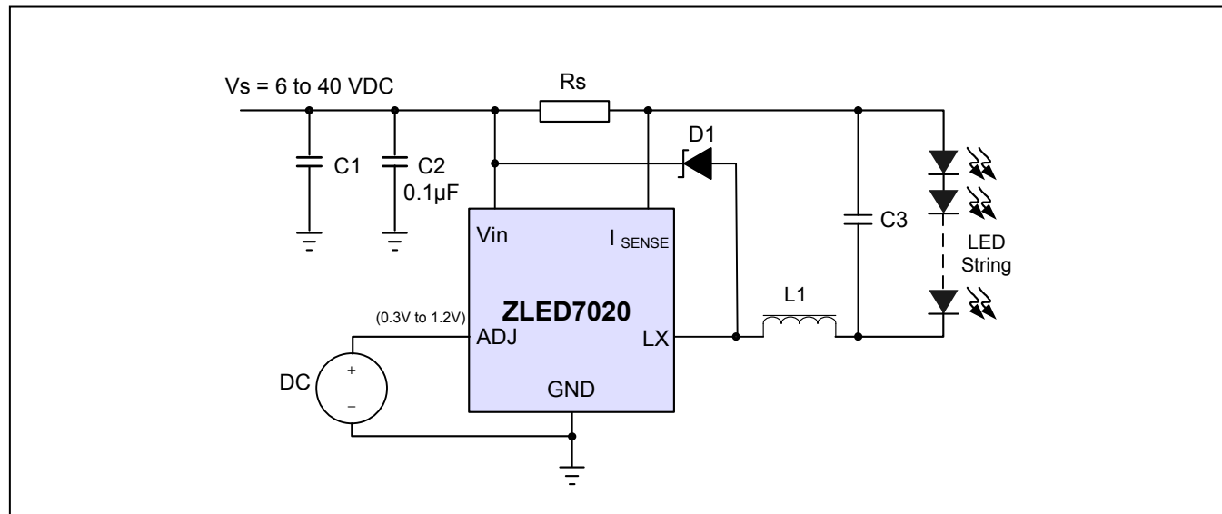
Figure 3.2 Basic ZLED7X20 Application Circuit with Output Current Controlled by External DC Voltage
