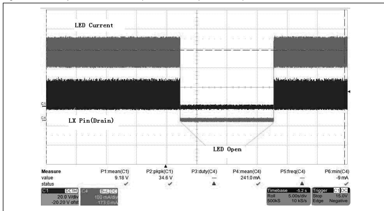
Figure 1.9 LED Open-Circuit Protection ( R_s=0.30\Omega , L_1=47\mu\text{H} , V_{IN}=24\text{ V} )
