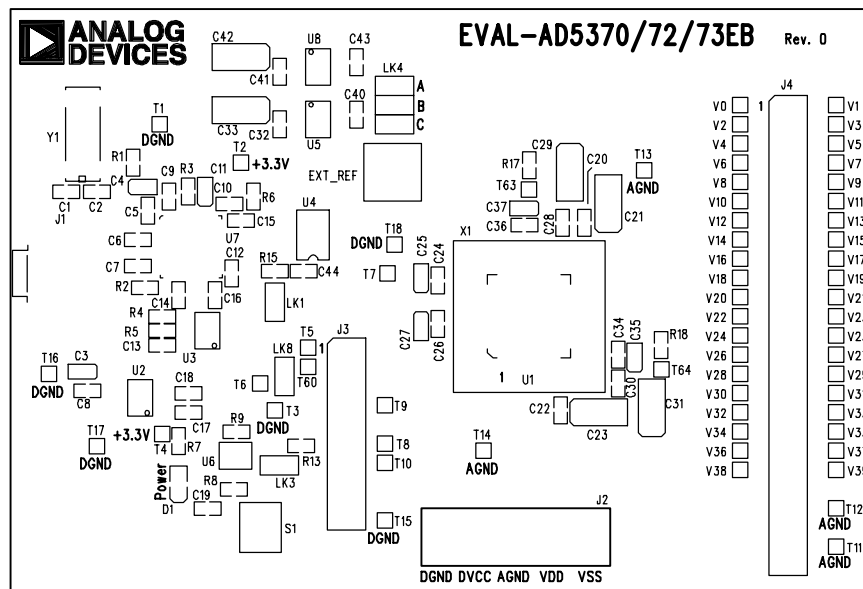
Eval-AD5370/72/73EB Rev. 0 (Component Side View)
