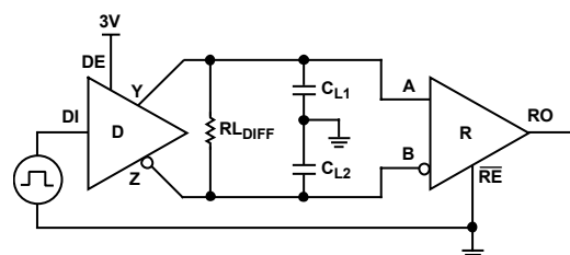
Figure 10. Driver/Receiver Propagation Delay Test Circuit
