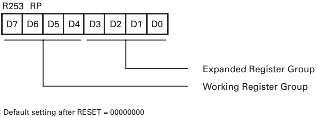
Figure 20. Register Pointer
