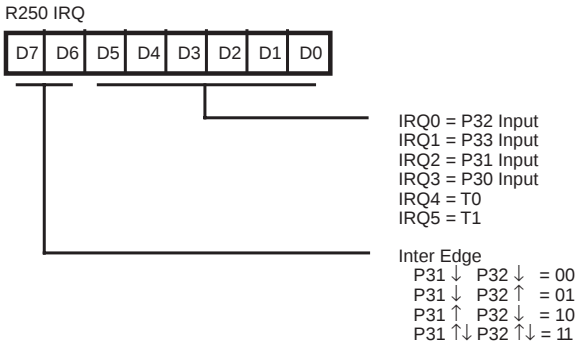
Figure 50. Interrupt Request Register (FA H : READ/WRITE)
