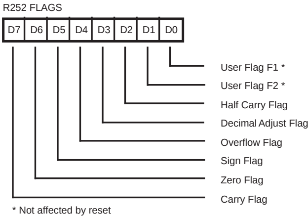
Figure 52. Flag Register (FC H : READ/WRITE)
