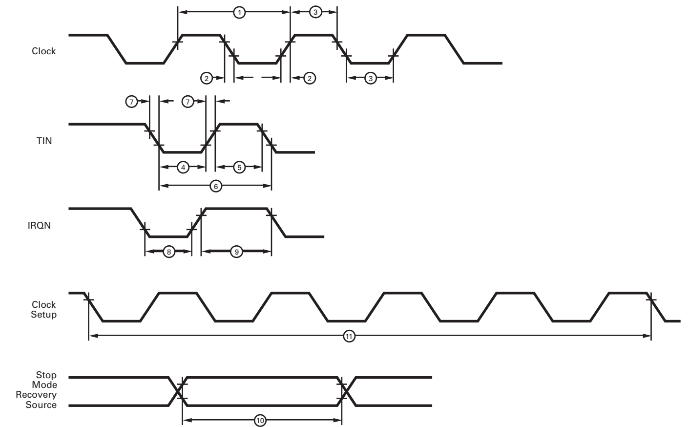
Figure 9. Additional Timing
