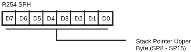
Figure 54. Stack Pointer High (FE H : READ/WRITE)
