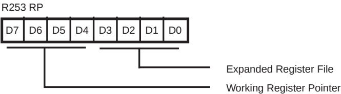
Figure 53. Register Pointer (FD H : READ/WRITE)
