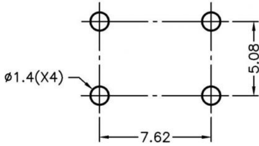
MOUNTING HOLES
