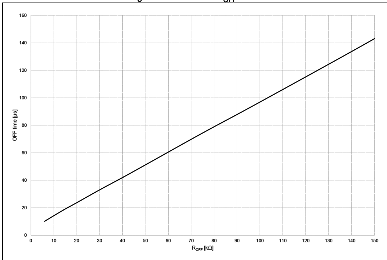
Figure 8. OFF time vs R_{\text{OFF}} value
