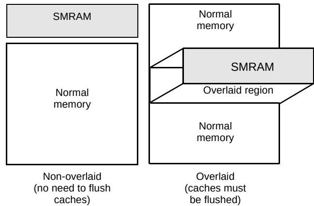
Figure 32. SMRAM Location
