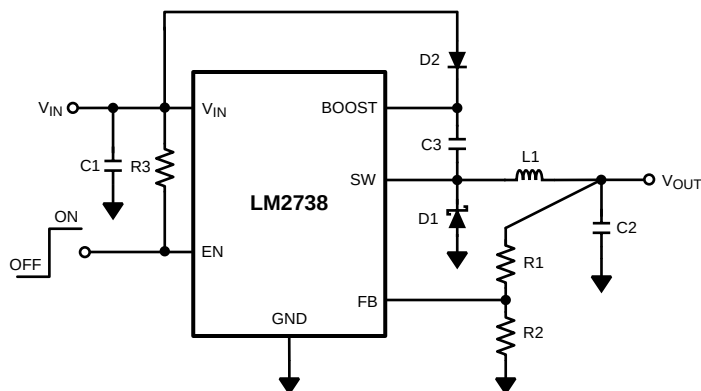
Figure 39. LM2738Y (550 kHz) V_{BOOST} Derived from V_{IN} 5 V to 1.5 V / 1.5 A
