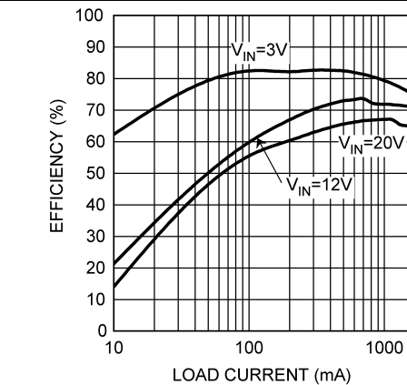
Figure 3. Efficiency vs Load Current – X Version
