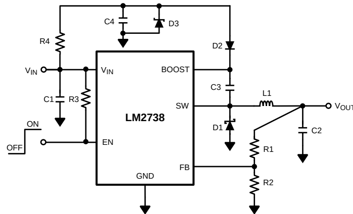
Figure 35. LM2738X (1.6 MHz) V_{\text{BOOST}} Derived from V_{\text{SHUNT}} 18 V to 1.5 V / 1.5 A
