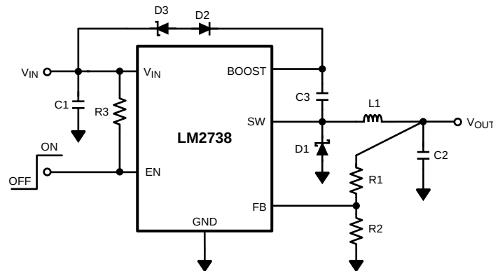
Figure 37. LM2738X (1.6 MHz) Derived from Series Zener Diode ( V_{IN} ) 15 V to 1.5 V / 1.5 A
