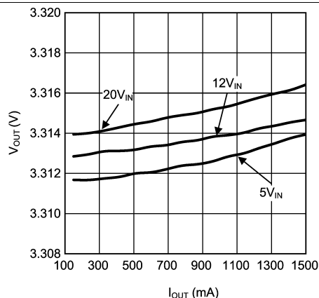
Figure 19. Load Regulation – X Version
