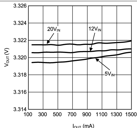
Figure 20. Load Regulation – Y Version
