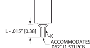
ACCOMMODATES .062" [1.57] PCB (CT, CS, CM, TK, CK, RS, RM) Example P/N: EBM10DCSN-S288 (Requires -S288 Modification Code)
