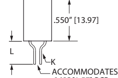
ACCOMMODATES .062" [1.57] PCB (KR, KN) Example P/N: EBM10DKRN (-S288 Not required)
