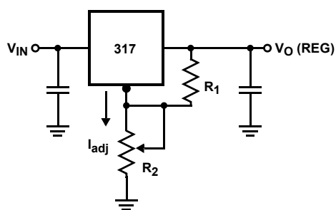
FIGURE 6. VOLTAGE REGULATOR
