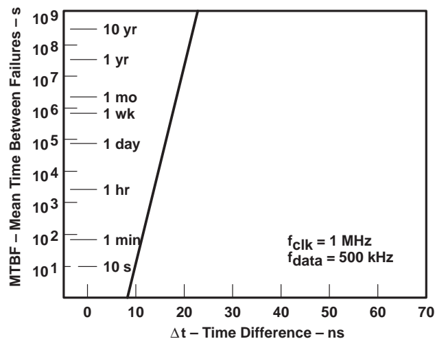
Figure 11. Metastable Characteristics
