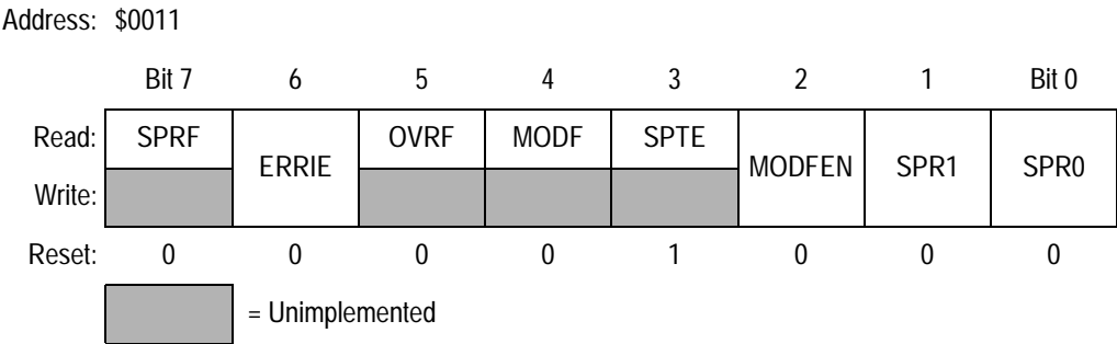
Figure 20-14. SPI Status and Control Register (SPSCR)
