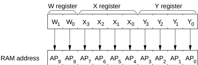
Register Direct Addressing
