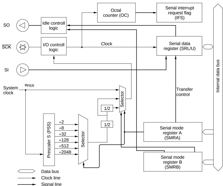
Figure 70 Block Diagram of Serial Interface
