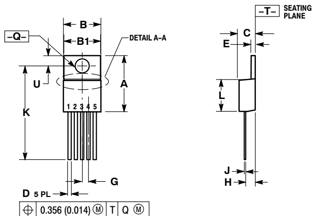
TO-220 5-LEAD CASE 314D-04 ISSUE H
