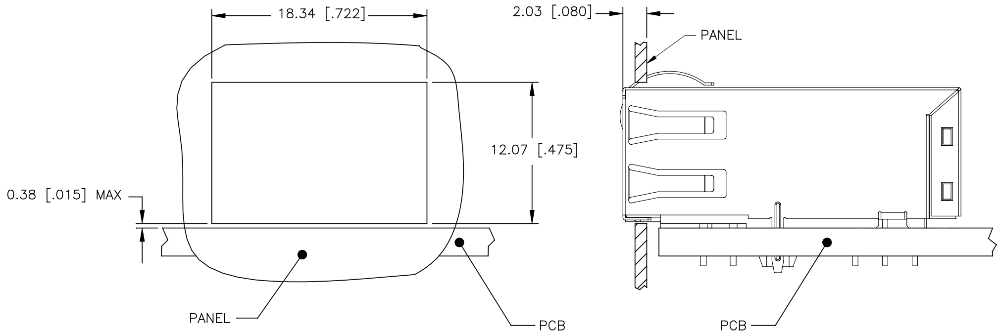
SUGGESTED PANEL CUTOUT
