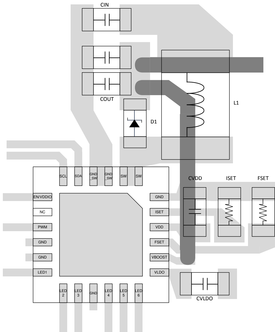
Figure 29. WQFN Layout
