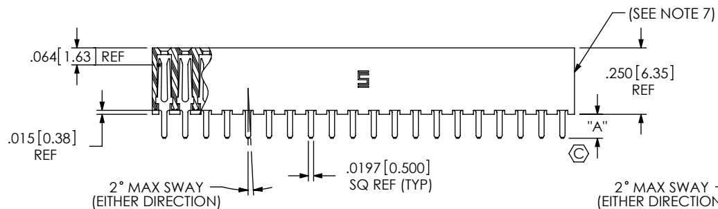
FIG 1 SQT-120-01-XX-6 SHOWN
